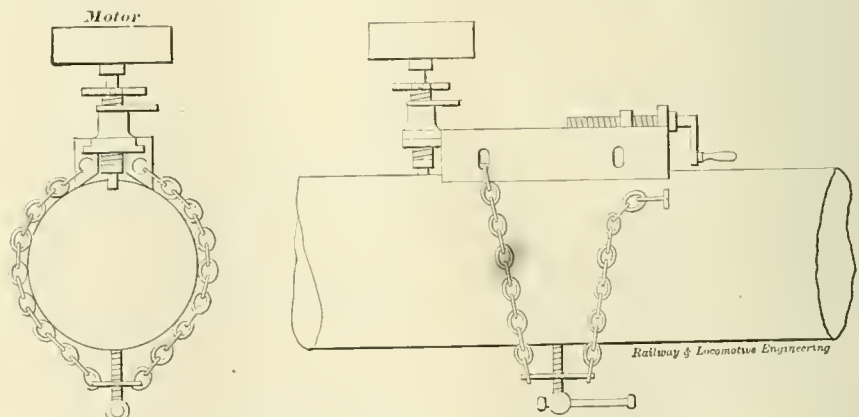
FIG. 3.—KEYWAY CUTTER OPERATED BY A MOTOR.
